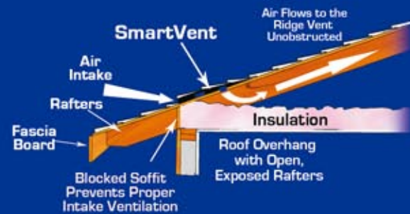
Mid-Roof Application
