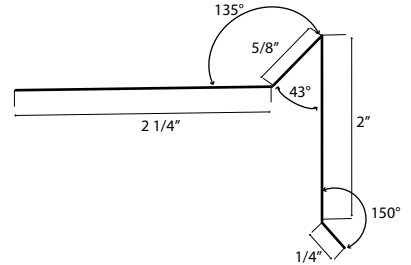
2" Gravel Stop
