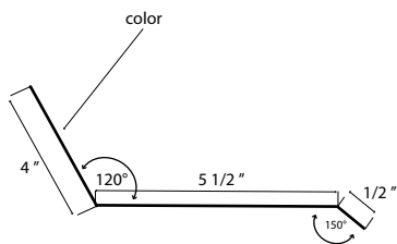
Roof to Wall w/ Kick
