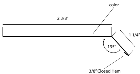
Starter 1 1/4"
