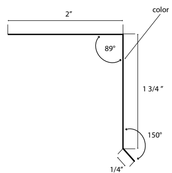
Drip 2"
