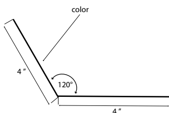
Roof to Wall w/ Kick
