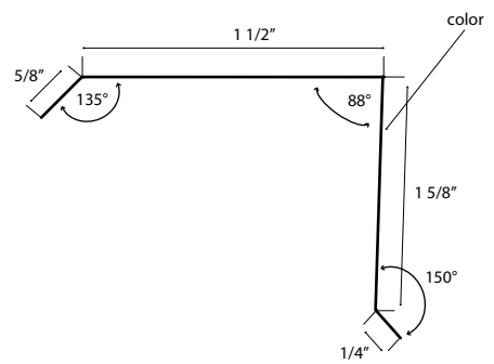
1 1/2" Fascia
