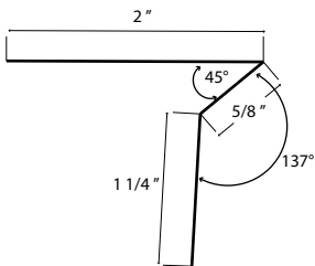
Big T metal
