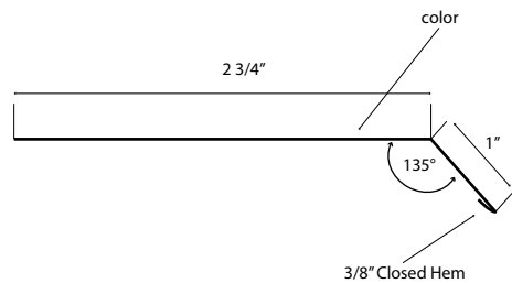
Starter 1"
