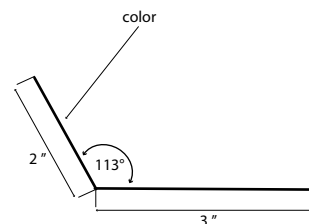
2 X 3 Roof to Wall
