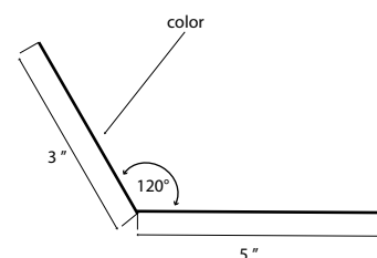
3X5 Roof to Wall
