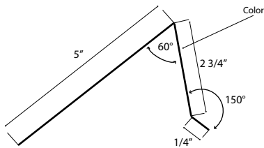
Clerestory
