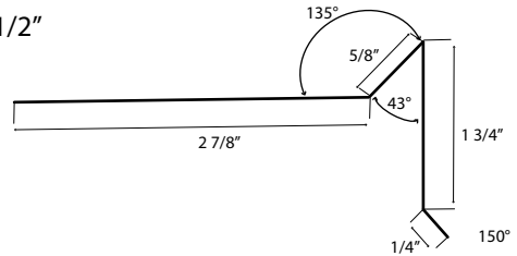
3" Gravel Stop
