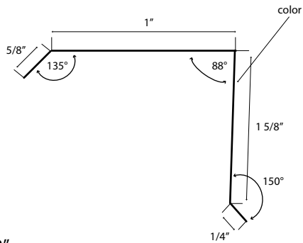
1" Fascia
