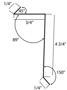
Chim 5"
