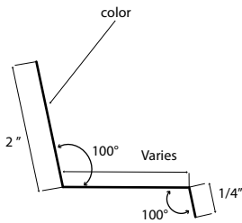
Fireplace Flashing
