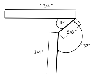
Small T Metal
