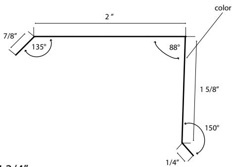
2" Fascia
