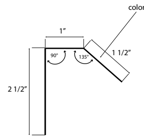
Re Roof Flashing
