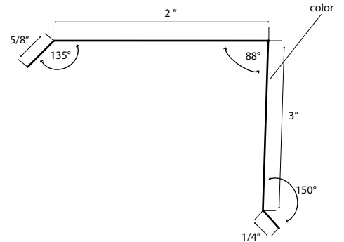
3" Fascia
