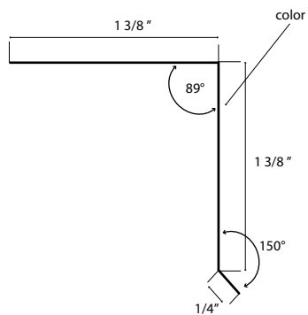
Drip 1 3/8"
